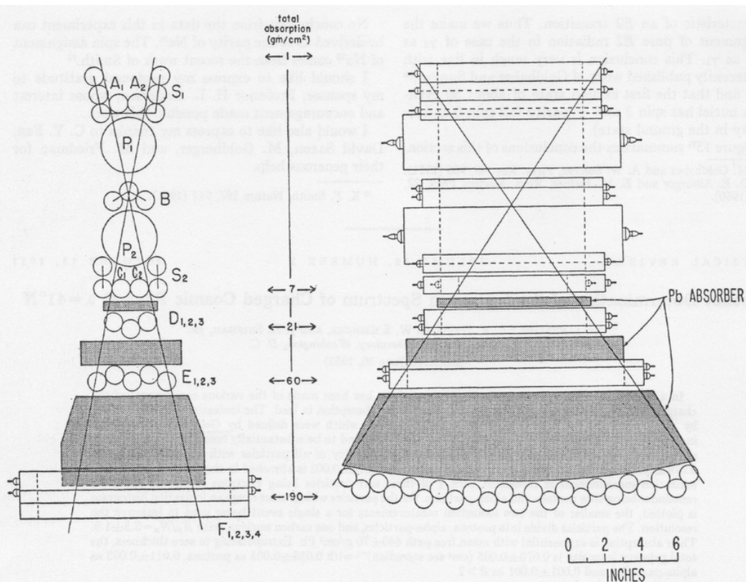
FIG. 1. Diagram of telescope.
