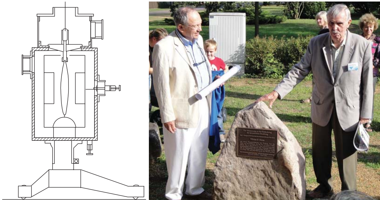
FIGURE 1. Left: Electrometer after Th. Wulf [5]. Right: Two grandchildren of V.F. Hess revealing a plaque to commemorate the discovery of cosmic rays on August 7th, 2012, close to the presumed landing site of V.F. Hess in Pieskow close to Berlin. It reads: "To commemorate the discovery of cosmic rays. On 7 August 1912 landed the Austrian physicist Victor F. Hess with a hydrogen balloon close to Pieskow. On the journey from Lower-Bohemia he reached an altitude of 5300 m and he proved the existence of a penetrating, ionizing radiation from outer space. For the discovery of cosmic rays V.F. Hess has been awarded the Nobel Prize in Physics in 1936. The participants of the symposium '100 years cosmic rays', Bad Saarow-Pieskow, 7 August 2012".
